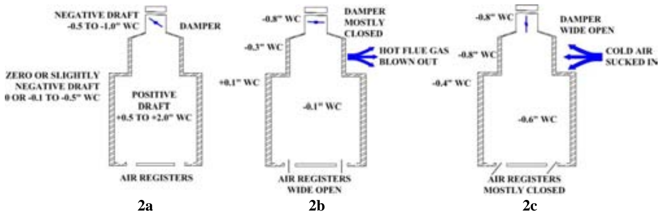
FIGURE 2 – ILLUSTRATION OF CORRECT AND INCORRECT DRAFT
